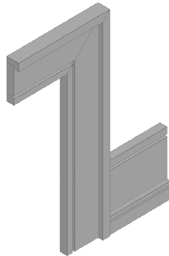
1006 - Casing 3 1/2" x 3/4" 1205 - Backband 1 1/4" x 3/4" with 3/4" rebate 1405 - Shoe Moulding & Doorstop 1 5/8" x 3/8" 1705 - Baseboard 7 1/4" x 3/4"
