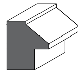
1202 - Backband 1 3/4" x 1 1/2" with 3/4" rebate
