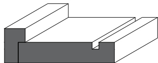
1006 - Casing 3 1/2" x 3/4" 1205 - Backband 1 1/4" x 3/4" with 3/4" rebate 1405 - Shoe Moulding & Doorstop 1 5/8" x 3/8" 1705 - Baseboard 7 1/4" x 3/4"
