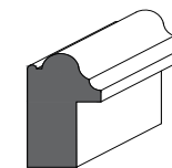
1214 - Backband 1 5/16" x 3/4" with 3/4" rebate
