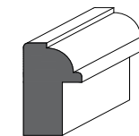
1213 - Backband 1 5/16" x 3/4" with 3/4" rebate
