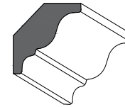
2601 - Crown Moulding 1 5/8" x 1/2" (A = 1 3/16") (B = 1 1/8")
