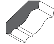
2603 - Crown Moulding 2 3/4" x 3/4" (A = 2") (B = 1 15/16")
