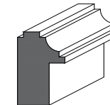
1210 - Backband 1 5/16" x 3/4" with 3/4" rebate
