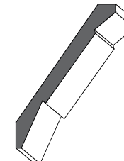
2608 - Crown Moulding 6 1/2" x 3/4" (A = 4 5/8") (B = 4 5/8")
