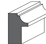
1211 - Backband 1 5/16" x 3/4" with 3/4" rebate
