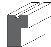
1216 - Backband 1 5/16" x 3/4" with 3/4" rebate
