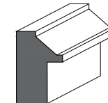
1209 - Backband 1 5/16" x 3/4" with 3/4" rebate
