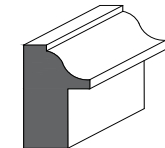
1212 - Backband 1 5/16" x 3/4" with 3/4" rebate
