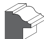
1207 - Backband 1 3/4" x 1 5/8" with 3/4" rebate
