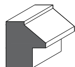
1202 - Backband 1 3/4" x 1 1/2" with 3/4" rebate
