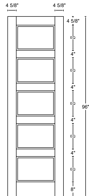
Front View
