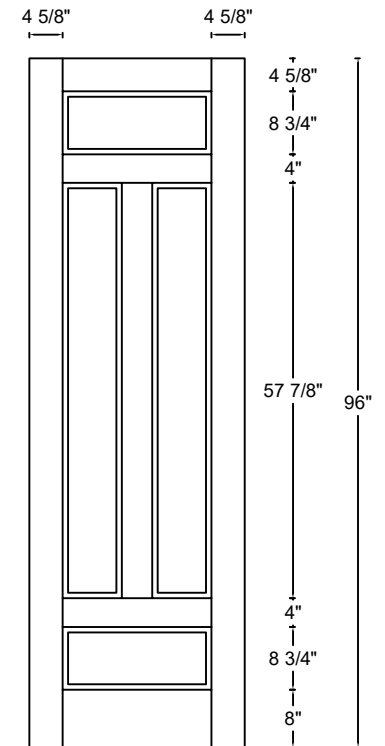
Front View
