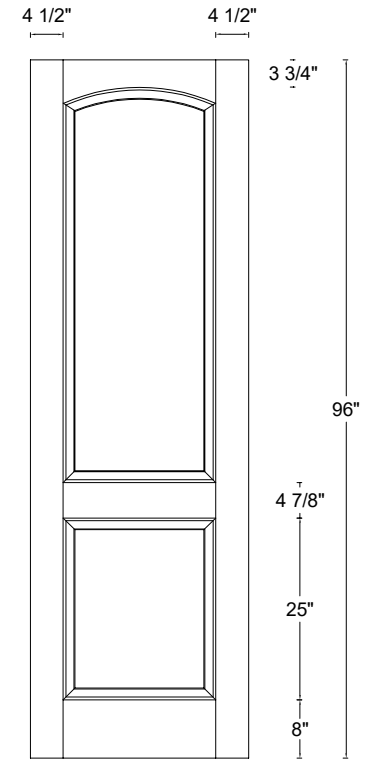
Front View
