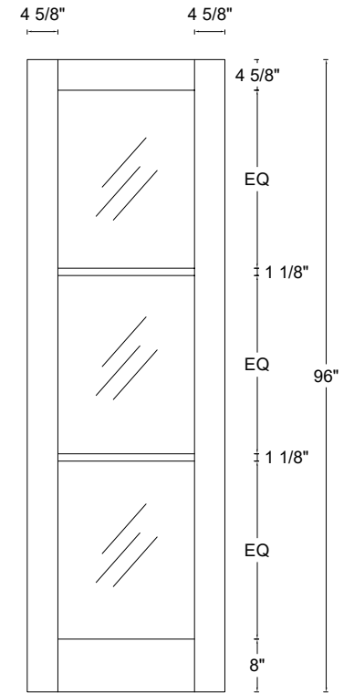
Front View
