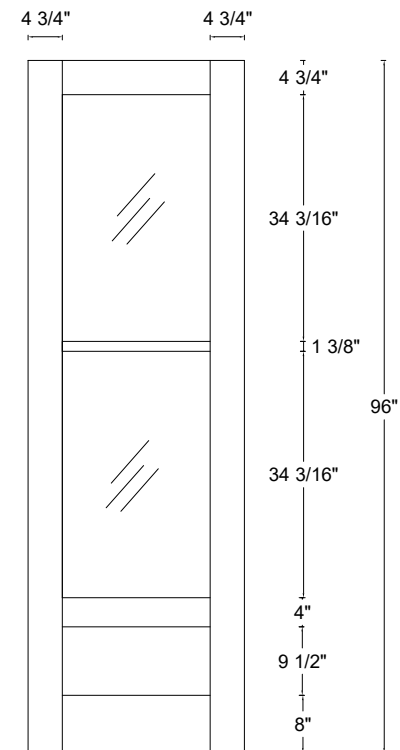
Front View
