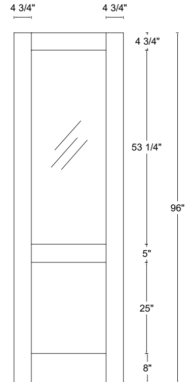
Front View
