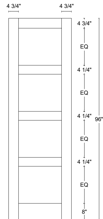
Front View
