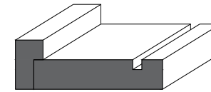
1006 - Casing 3 1/2" x 3/4" 1205 - Backband 1 3/4" x 3/4" with 3/4" rebate 1405 - Shoe Moulding & Doorstop 1 5/8" x 3/8" 1905 - Baseboard 9 1/4" x 3/4"
