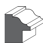
1207 - Backband 1 3/4" x 1 5/8" with 3/4" rebate
