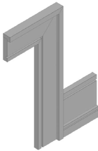
1006 - Casing 3 1/2" x 3/4" 1205 - Backband 1 3/4" x 3/4" with 3/4" rebate 1405 - Shoe Moulding & Doorstop 1 5/8" x 3/8" 1705 - Baseboard 7 1/4" x 3/4"
