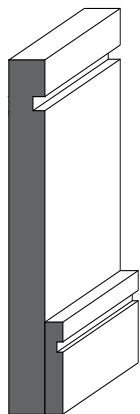
1006 - Casing 3 1/2" x 3/4" 1205 - Backband 1 3/4" x 3/4" with 3/4" rebate 1405 - Shoe Moulding & Doorstop 1 5/8" x 3/8" 1705 - Baseboard 7 1/4" x 3/4"
