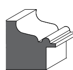
1208 - Backband 1 11/16" x 1 11/16" with 3/4" rebate
