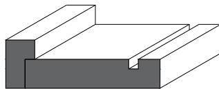
1006 - Casing 3 1/2" x 3/4" 1205 - Backband 1 3/4" x 3/4" with 3/4" rebate 1405 - Shoe Moulding & Doorstop 1 5/8" x 3/8" 1705 - Baseboard 7 1/4" x 3/4"
