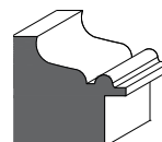
1208 - Backband 1 11/16" x 1 11/16" with 3/4" rebate
