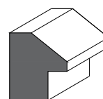
1204 - Backband 1 3/4" x 1 1/2" with 3/4" rebate
